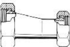
32-14F Eccentric Taper Reducer
